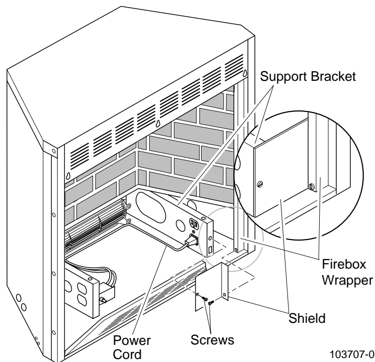
Figure 2 - Installing Shield
