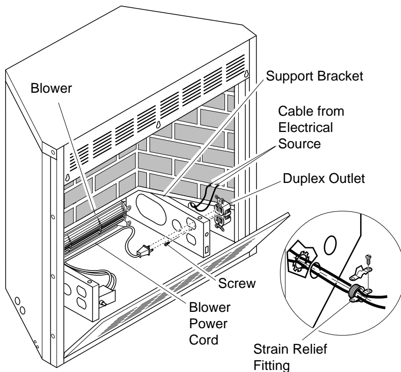
Figure 1 - Installing Duplex Outlet
